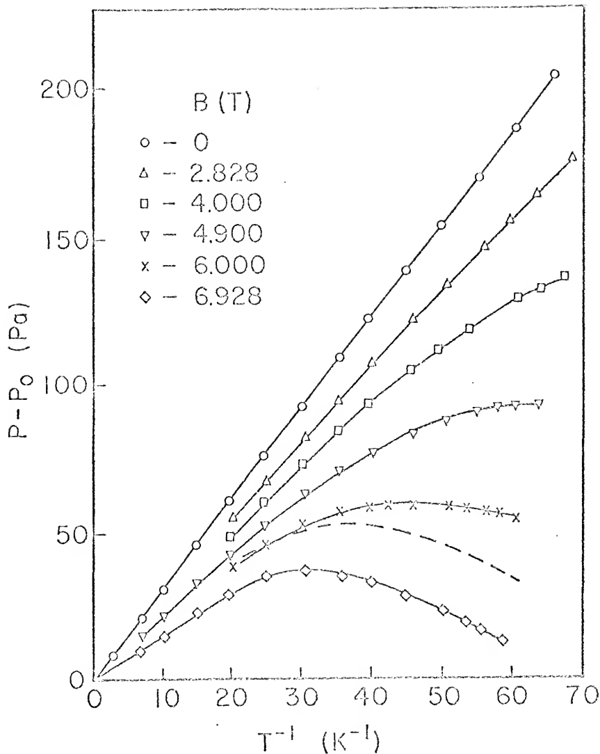
Fig. 10 Pressure Change with Temperature for Various Fields.
